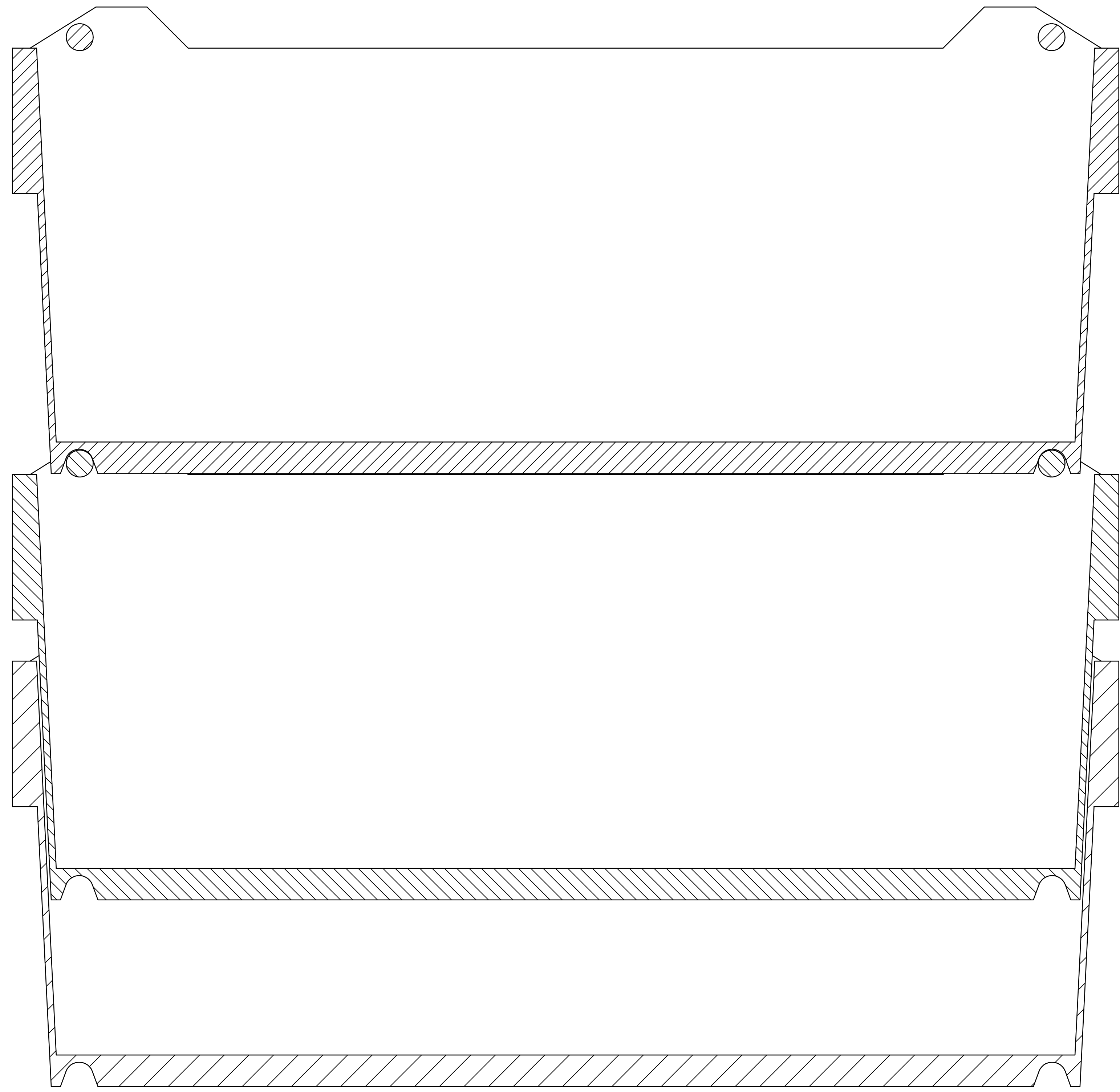
SECTION C-C
