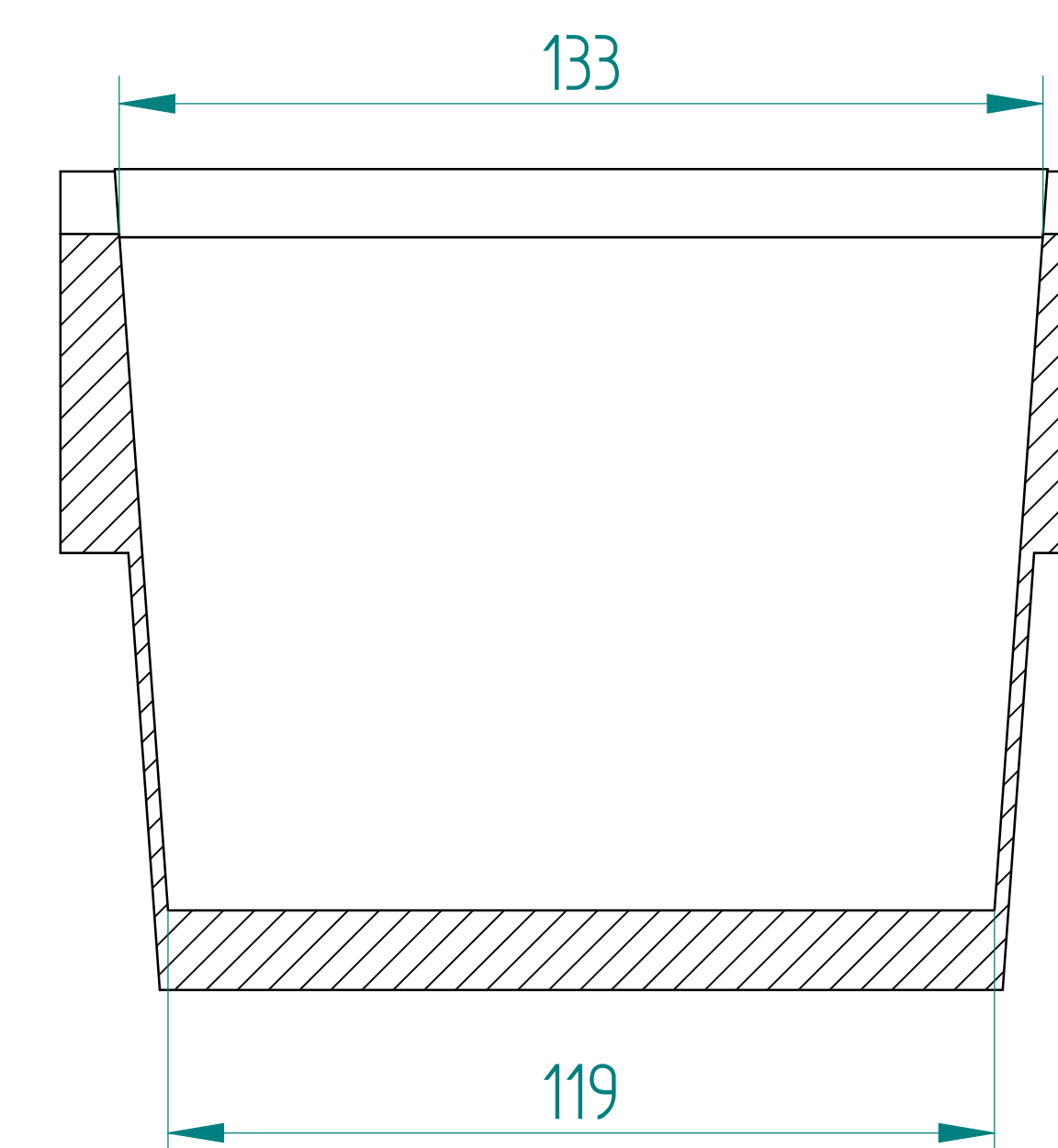
SECTION B-B
